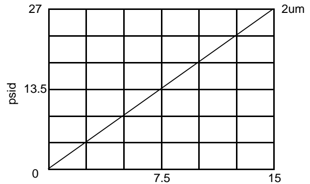
150 SUS, 0.9 SG Fluid Pressure drop varies linearly with viscosity.
