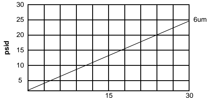
150 SUS, 0.9 SG Fluid Pressure drop varies linearly with viscosity.
