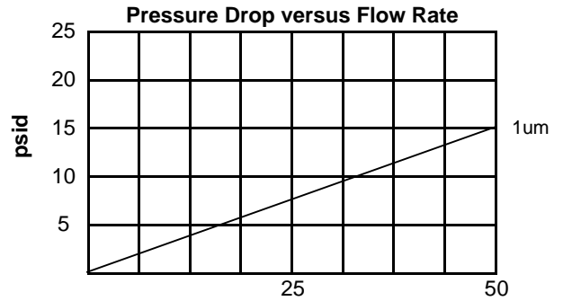
GPM - 150 SUS, 0.9 SG Fluid Pressure drop varies linearly with viscosity.
